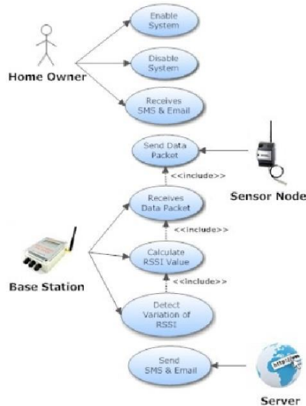
Figure 1.4: Intelligent Home Monitoring Using RSSI in Wireless Sensor Networks.
